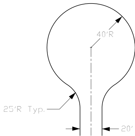
80' Diameter Cul-de-Sac
