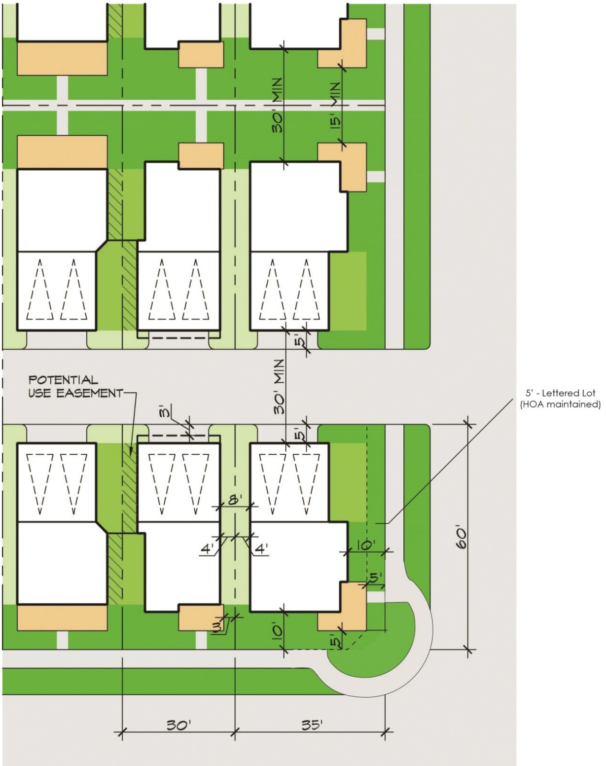
ALLEY LOADED SINGLE FAMILY DETACHED
