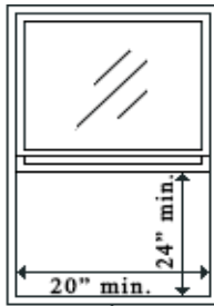
SINGLE HUNG Clear opening must be 5.7 ft 2 , or 5 ft 2 if grade floor opening.
