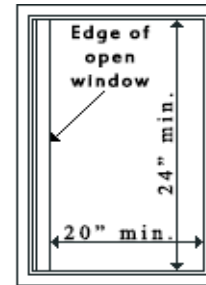
CASEMENT Clear opening must be 5.7 ft 2 , or 5 ft 2 if grade floor opening.
