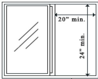
SLIDER Clear opening must be 5.7 ft 2 , or 5 ft 2 if grade floor opening.
