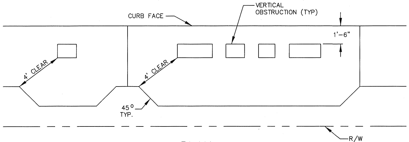
PLAN
