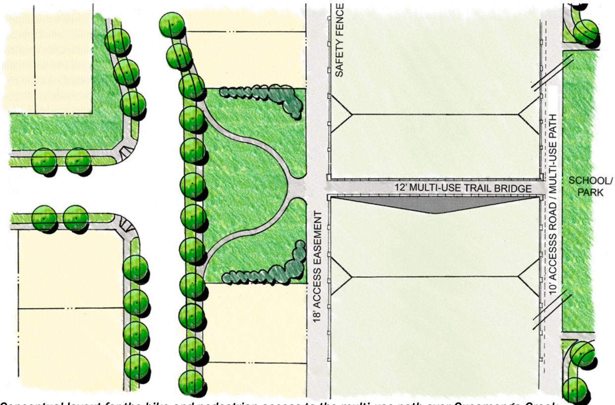
Conceptual layout for the bike and pedestrian access to the multi-use path over Cucamonga Creek
